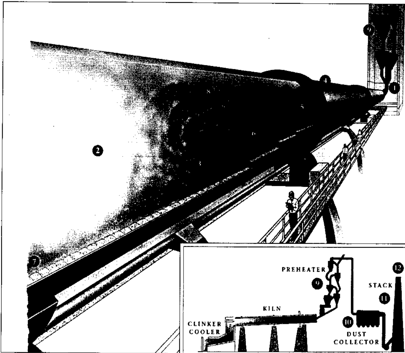
Figure 1 - Preheater Dry Process Cement Kiln
